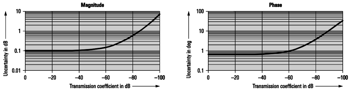
Typical accuracy of transmission magnitude and transmission phase measurements of the R&S®ZVT20 in the frequency range from 10 MHz to 700 MHz
