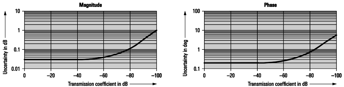
Typical accuracy of transmission magnitude and transmission phase measurements of the R&S®ZVT20 in the frequency range from 700 MHz to 20 GHz
