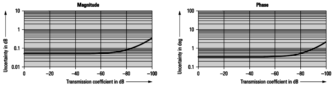
of the R&S®ZVT8 in the frequency range from 4 GHz to 8 GHz
