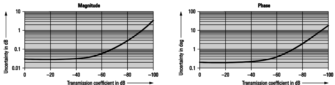
Typical accuracy of transmission magnitude and transmission phase measurements of the R&S®ZVT8 in the frequency range from 300 kHz to 4 GHz
